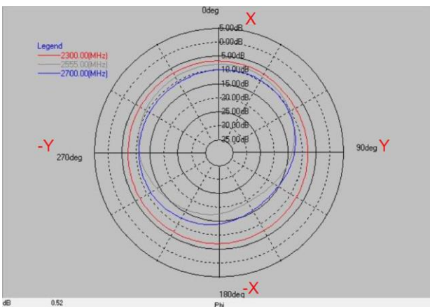
Frequency(MHz) : 2300~2700. Pattern Field : X-Y plane
