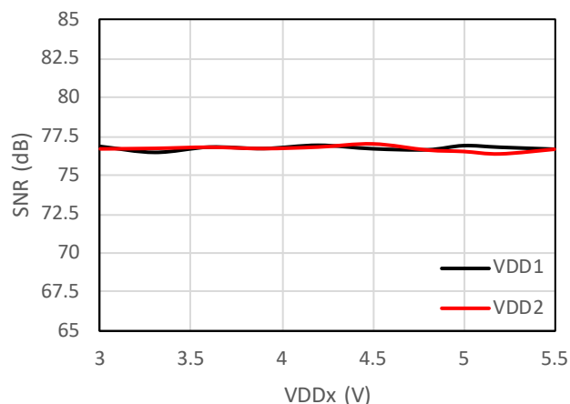
图 7-10 信噪比 vs 供电电压 @ f_{IN} = 1 kHz
