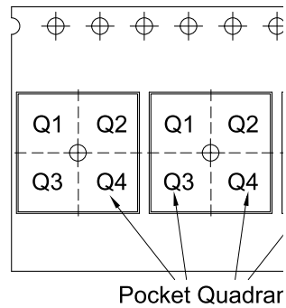
QUADRANT ASSIGNMENTS FOR PIN 1 ORIENTATION IN TAPE
