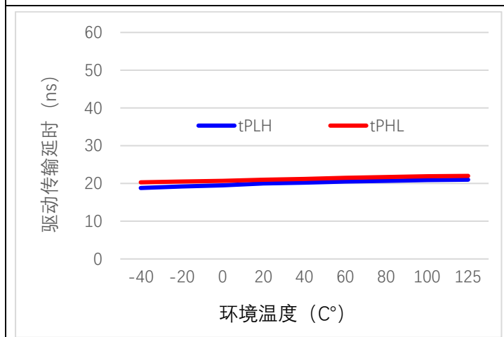
图 7.10-9 CA-IS3092x 驱动传输延时, V_{CC} = 3.3V , V_{ISO} = 3.3V , R_L = 54\Omega
