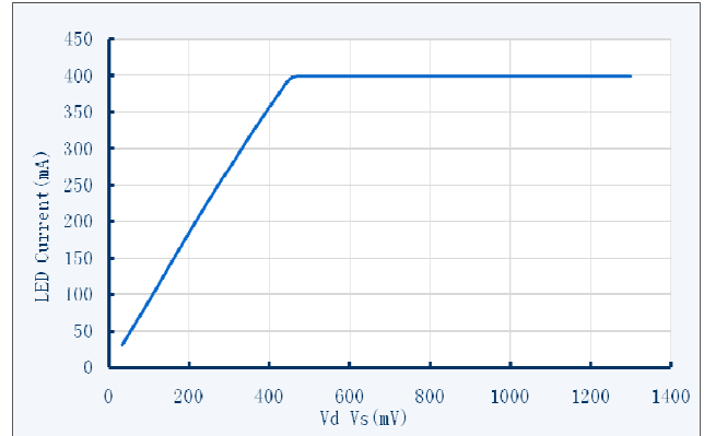
LED current vs. LED pin voltage
