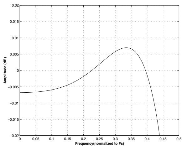
Figure 27. Single-Speed (slow) Passband Ripple
