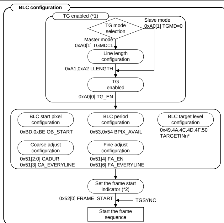
Figure 42 BLC Configuration
