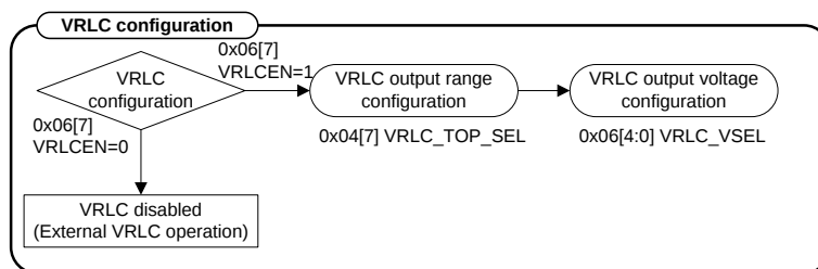
Figure 40 VRLC Configuration
