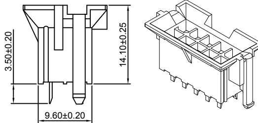
P/N: C4201WVD-F1-2xXP
