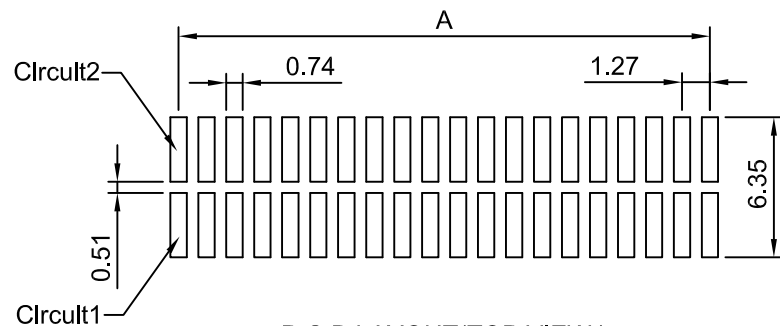
P.C.B LAYOUT (TOP VIEW) TOLERANCE: ±0.05
