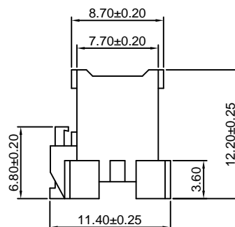
2x4P~2x8P
