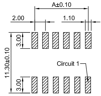
P.C.B LAYOUT TOLERANCE:±0.05
