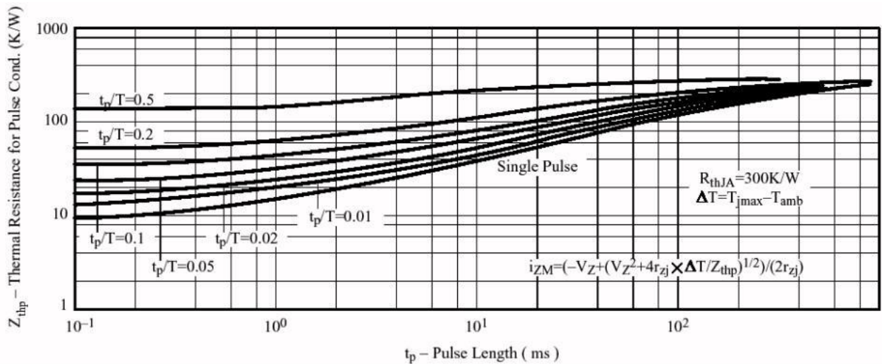
Figure 10. Thermal Response
