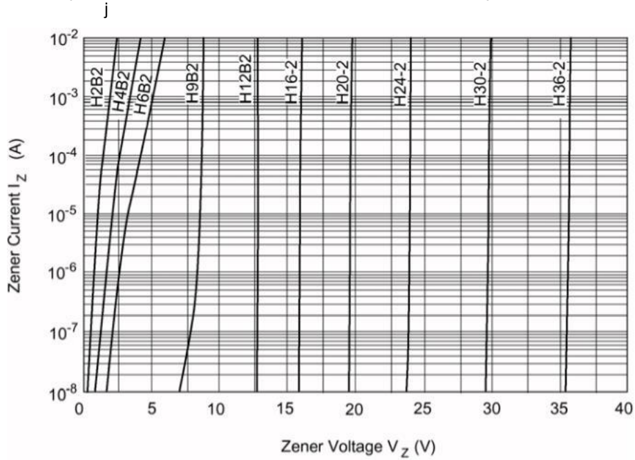
Figure 1. Zener current vs. zener voltage
