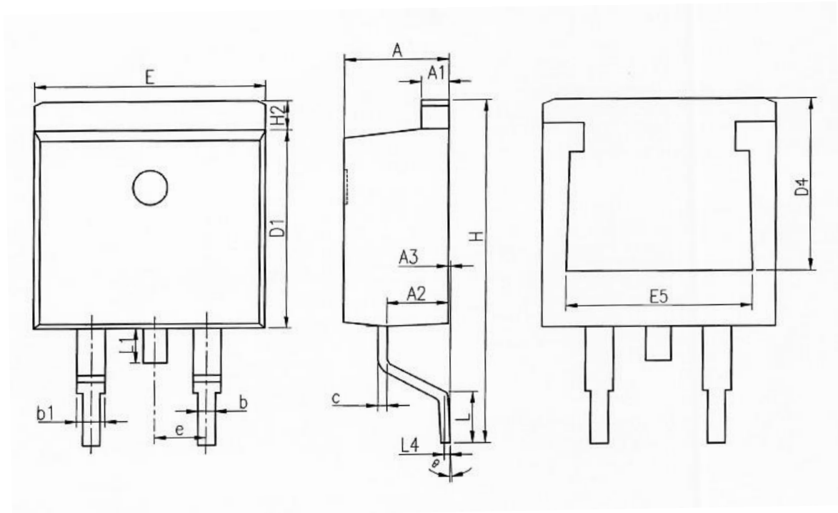
Figure 2 Outline TO-263 Dimensions in mm
