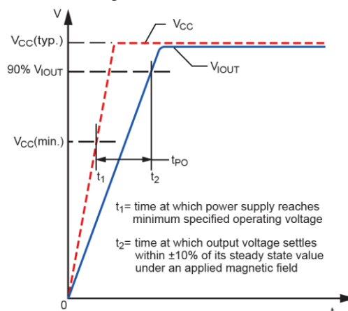
Figure 4: Power-On Time
