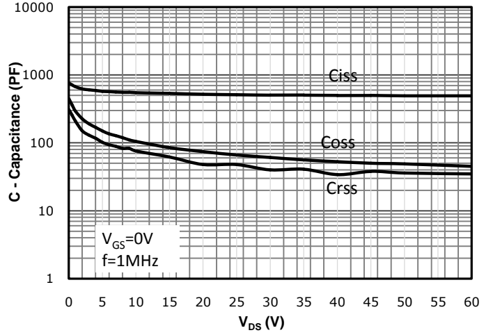
Fig 6: Capacitance Characteristics
