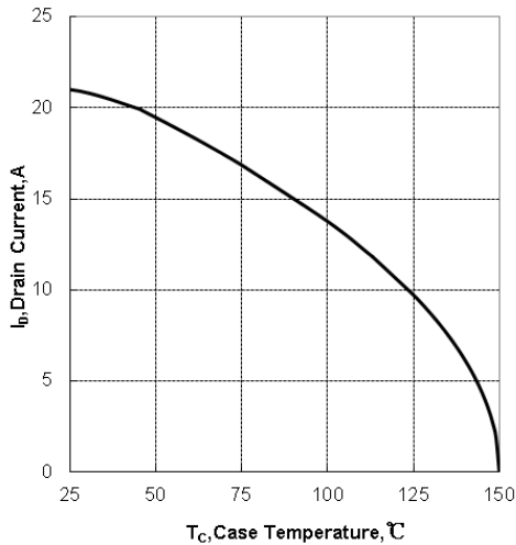
Figure 3. Maximum Continuous Drain Current vs Case Temperature
