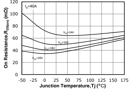
Fig 6: R DS(on) vs. Temperature For Various Gate Voltage
