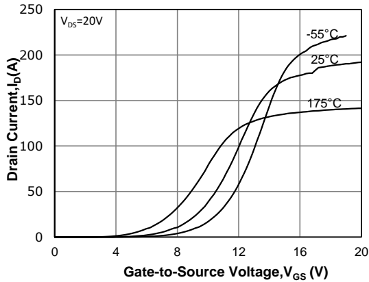
Fig 7: Transfer Characteristics
