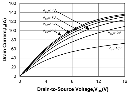
Fig 3. Output Characteristics (T j =175°C)
