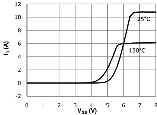
Fig 3: Transfer Characteristics
