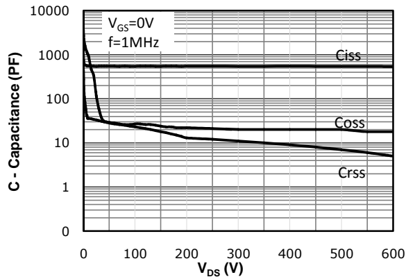
Fig 11: Capacitance Characteristics
