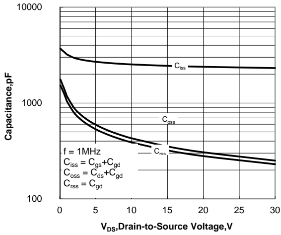
Figure 12. Capacitance Characteristics
