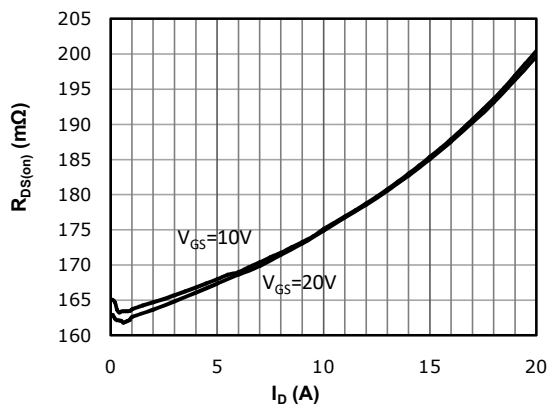
Fig 5: R DS(on) Vs Ids Characteristics
