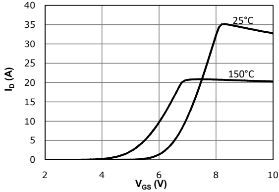
Fig 3: Transfer Characteristics
