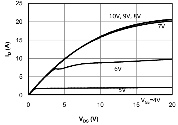
Fig 2. Output Characteristics (Tj=150°C)
