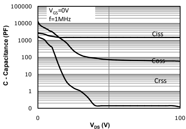
Fig 11: Capacitance Characteristics
