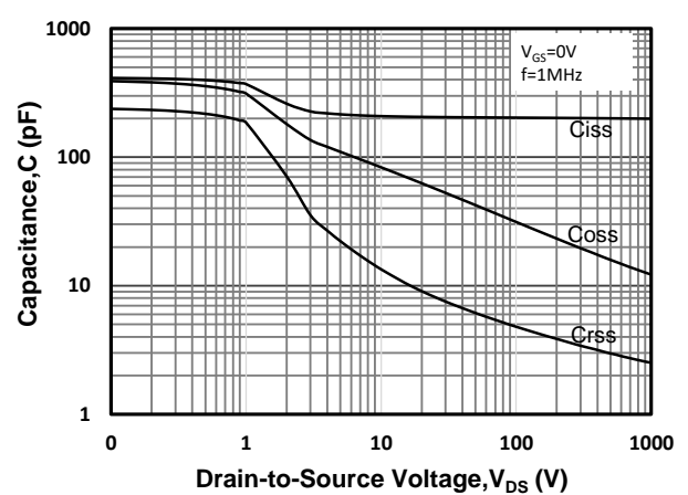
Fig 12: Capacitance Characteristics
