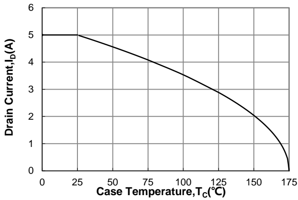
Fig 13: Continuous Drain Current vs. Case Temperature
