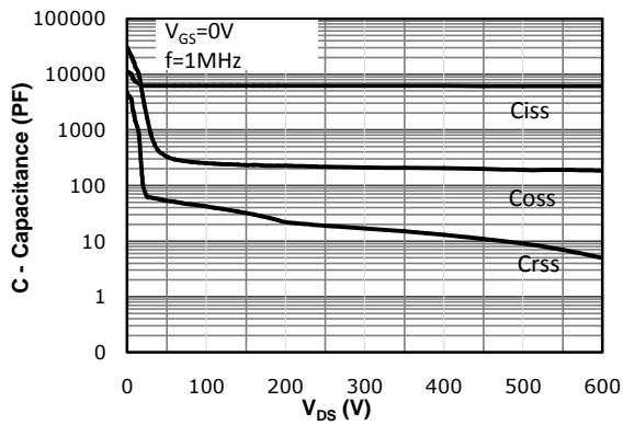
Fig 11: Capacitance Characteristics
