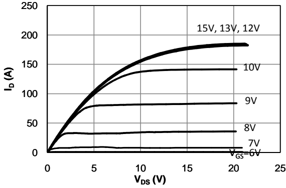
Fig 1. Output Characteristics (Tj=25°C)
