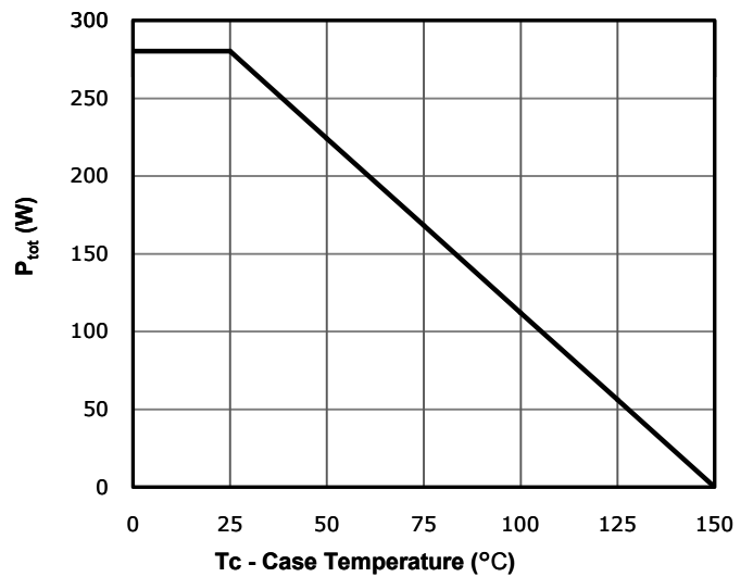
Fig 10: Power Dissipation
