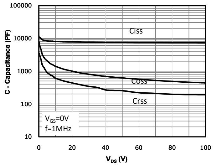
Fig 8: Capacitance Characteristics
