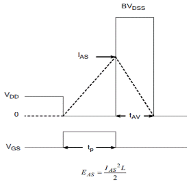
Figure 21. Unclamped Inductive Switching
