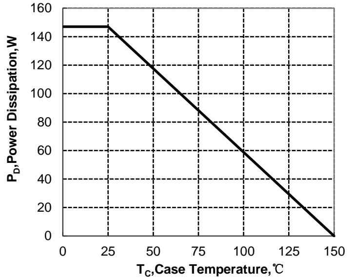
Figure 2. Maximum Power Dissipation vs Case Temperature
