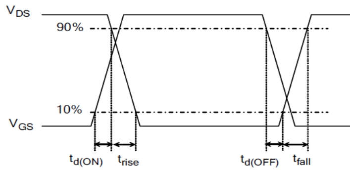
Figure 17. Resistive Switching
