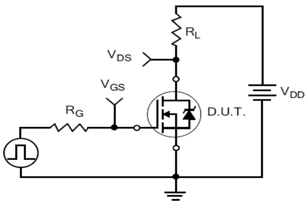
Figure 16. Resistive Switching Test Circuit Waveforms
