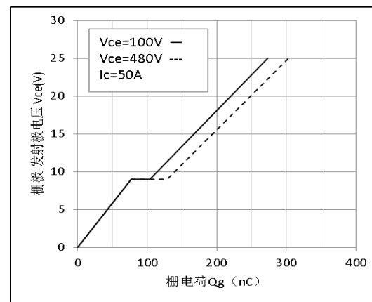
Figure 18.Gage Charge Characteristics
