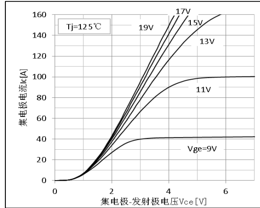
Figure 2.Output Characteristics
