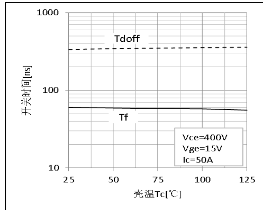
Figure 10.Switching Time-T c Characteristics
