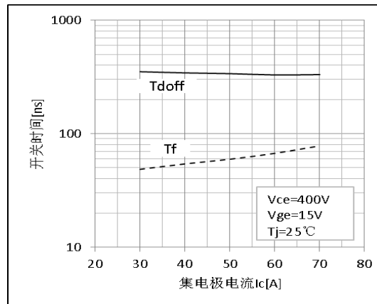
Figure 14.Switching Time-Ic Characteristics
