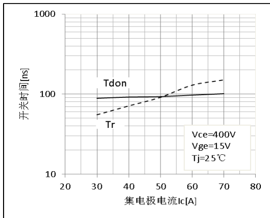
Figure 13.Switching Time-Ic Characteristics
