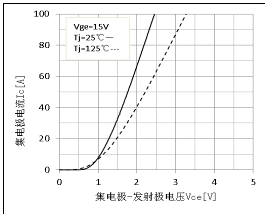
Figure 3.Saturation Voltage Characteristics
