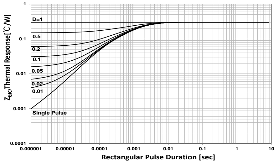
Figure 19.IGBT Transient Thermal Impedance
