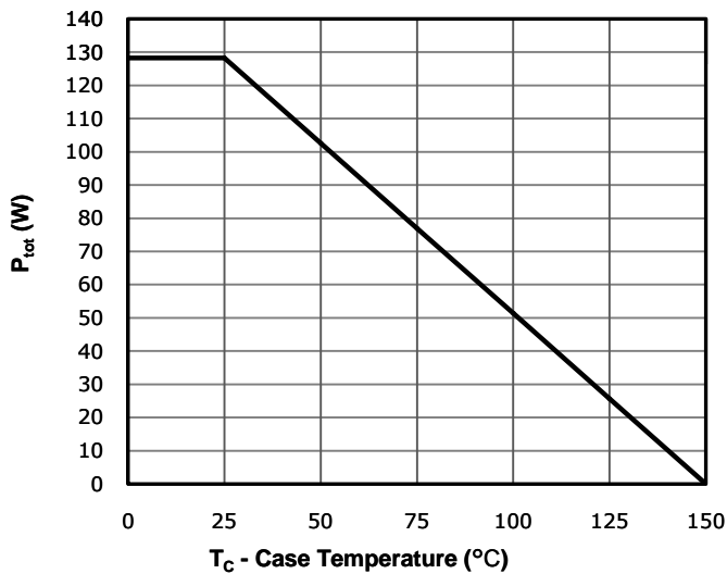
Fig 9: Power Dissipation
