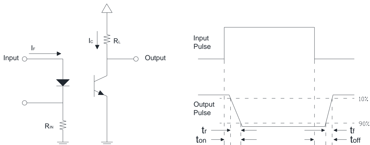
Figure 11: Switching Time Test Circuits
