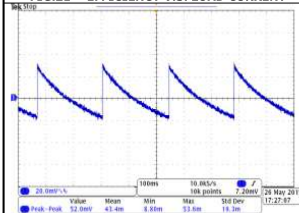
FIG.23 OUTPUT RIPPLE (12VIN, 2.5VOUT, IOUT=0A)
