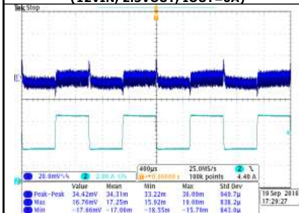
FIG.25 TRANSIENT RESPONSE (12VIN, 2.5VOUT, 50% to 100% LOAD STEP)
