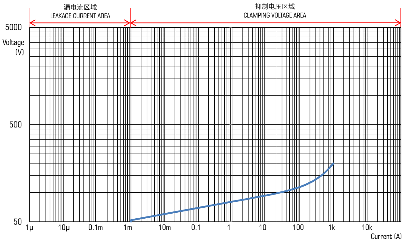
Typical 14D470K clamping voltage characteristic curve (for reference)
