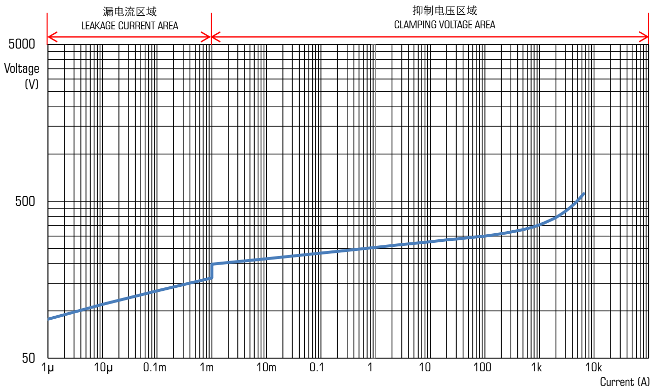
Typical 20D181K clamping voltage characteristic curve (for reference)
