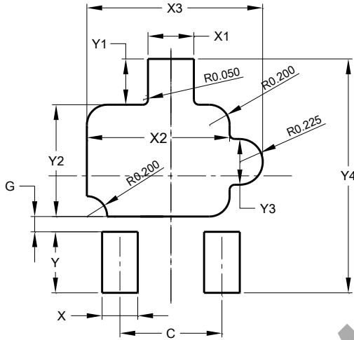
U-DFN2020-3
