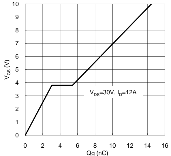
Figure 10. Gate Charge
