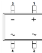
Pin Diagram
