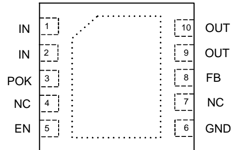
DFN3030-10
