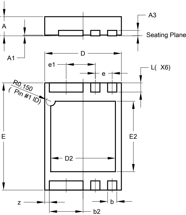
U-DFN2535-6(Type B)
