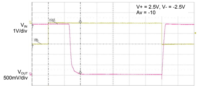
Time 50μs/div
