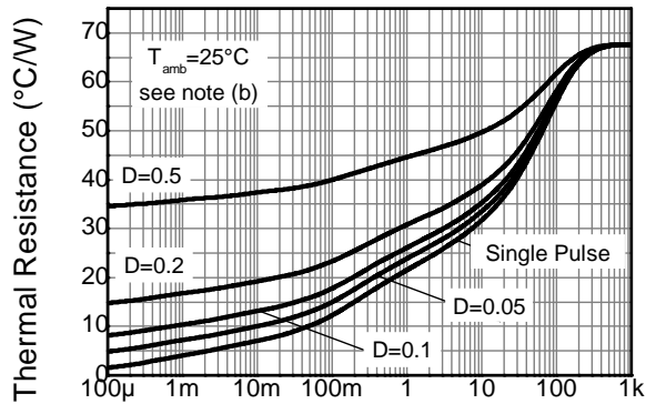
Pulse Width (s) Transient Thermal Impedance
