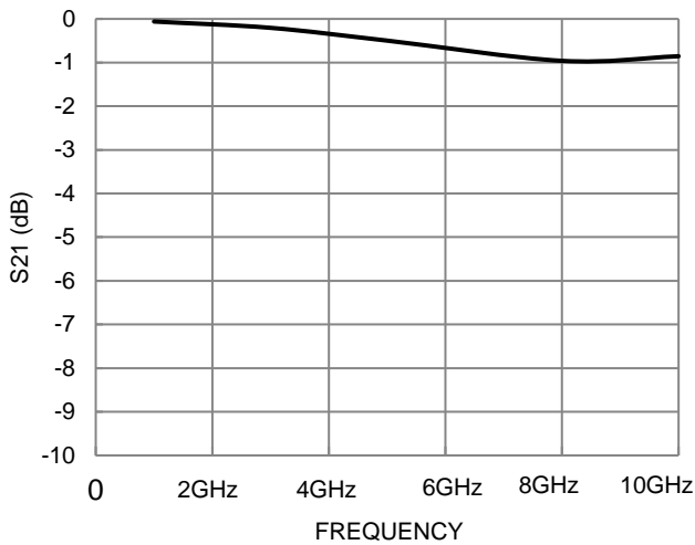
Figure 5 S21(dB) Attenuation Measurement
