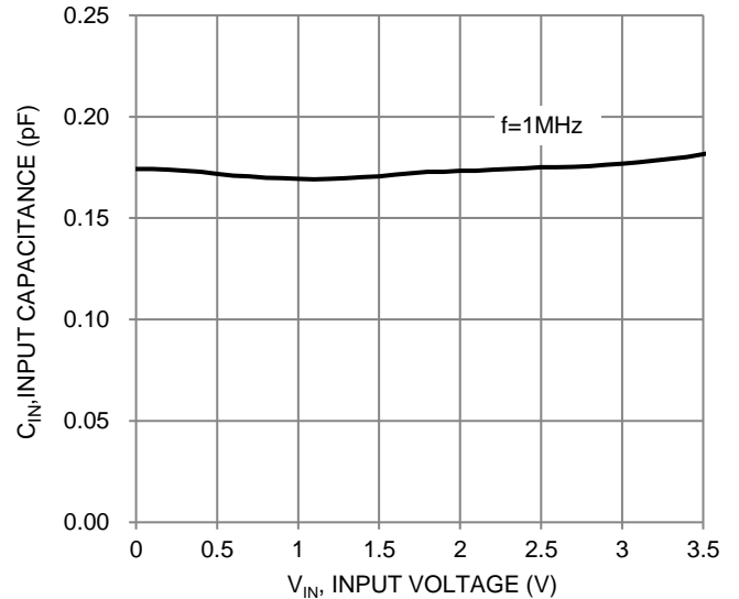
Figure 4 Input Capacitance vs. Input Voltage
