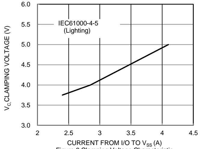
Figure 6 Clamping Voltage Characteristic
