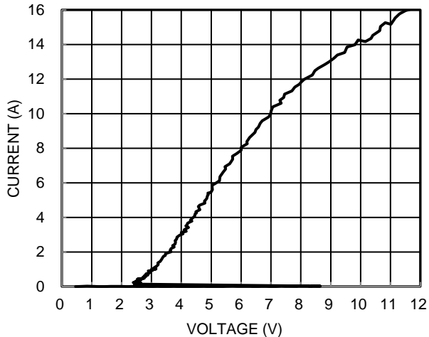
Figure 7 Current vs. Voltage
