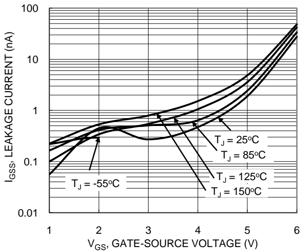
Figure 11. Gate-Source Leakage Current vs. Voltage
