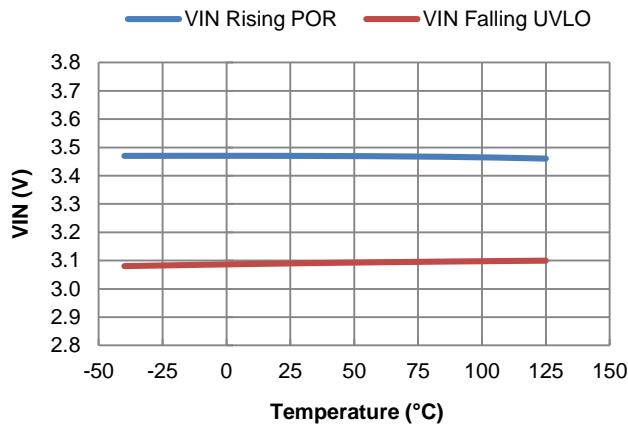
Figure 12. V IN Power-On Reset and UVLO vs. Temperature
