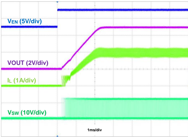
Figure 21. Startup Using EN, IOU = 2A
