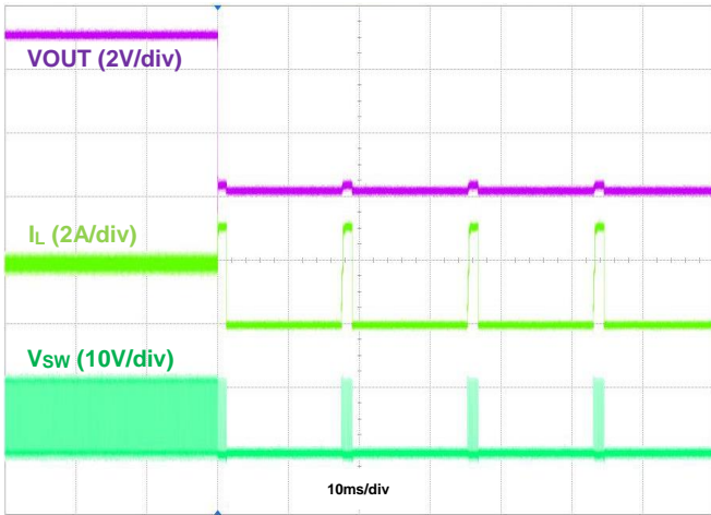
Figure 23. Output Short Protection, IOU = 2A
