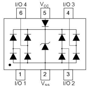
Device Schematic
