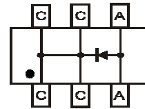
Top View Internal Schematic Dot denotes cathode pin 1
