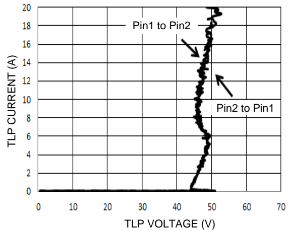
Figure 6 TLP Curve (tp=100ns)
