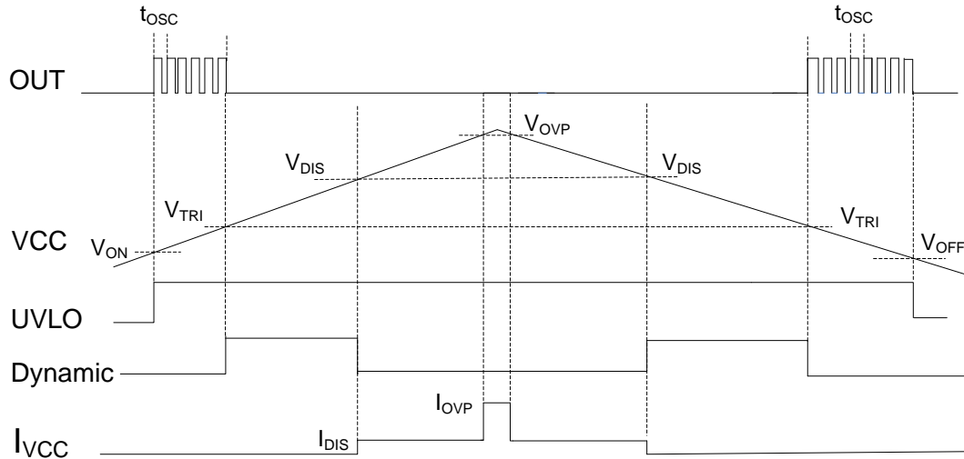
Figure 1. Typical Waveforms of AP4340S
