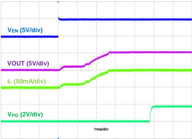
Figure 10. Startup Using EN, IOUT = 50mA
