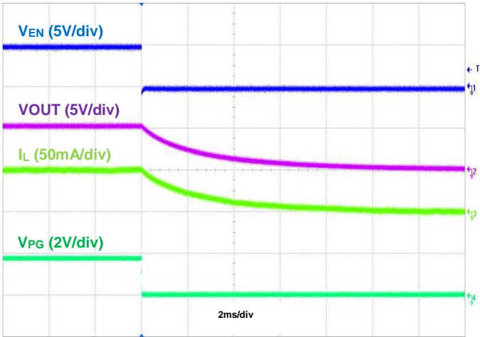
Figure 11. Shutdown Using EN, IOUT = 50mA
