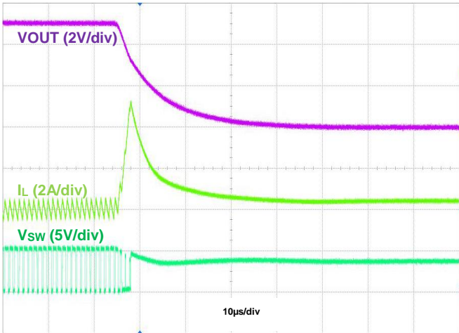
Figure 12. Output Short Protection, IOUT = 0A
