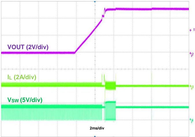
Figure 13. Output Short Recovery, IOUT = 0A
