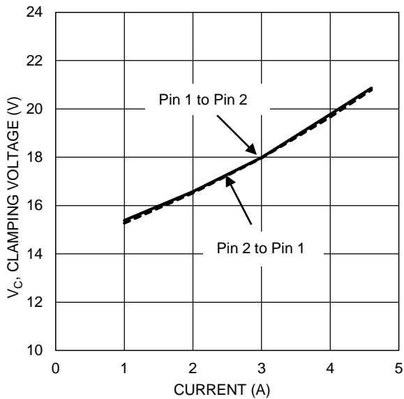
Figure 5 Clamping Voltage Characteristic (t p = 8/20μs)
