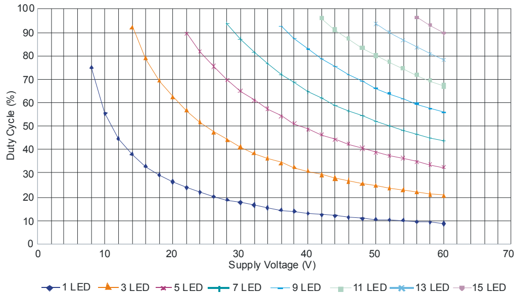
ZXLD1362 Duty Cycle L = 68μH
