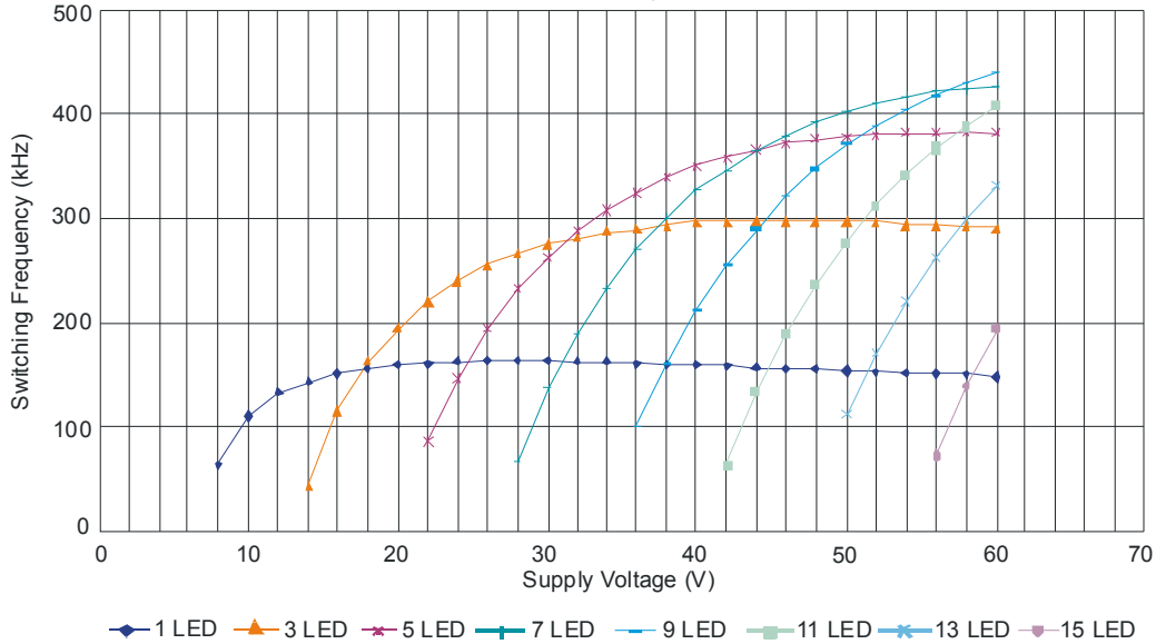
ZXLD1362 Switching Frequency L = 68μH
