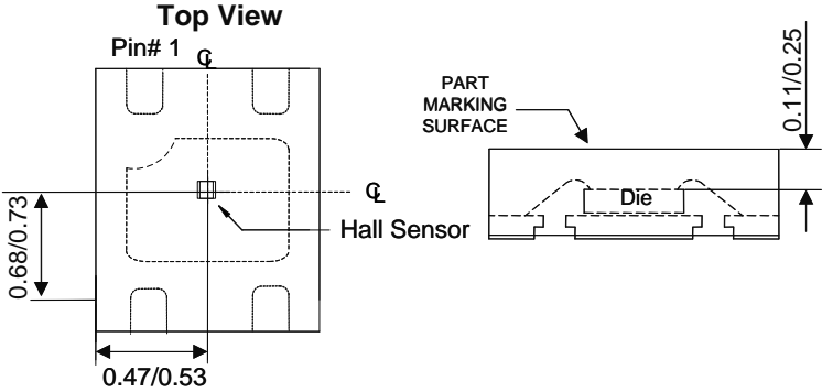
Sensor Location
