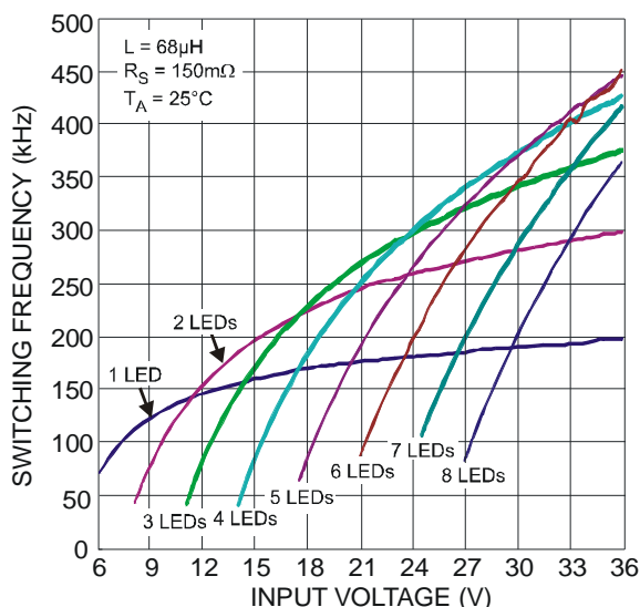
Figure 21 Switching Frequency vs. Input Voltage
