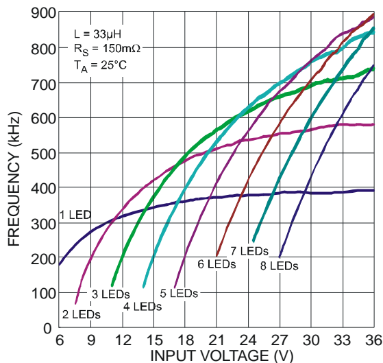
Figure 23 Switching Frequency vs. Input Voltage
